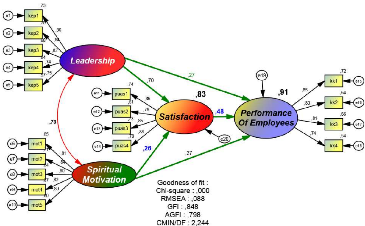
Figure 2. Output Effect Analysis by SEM
